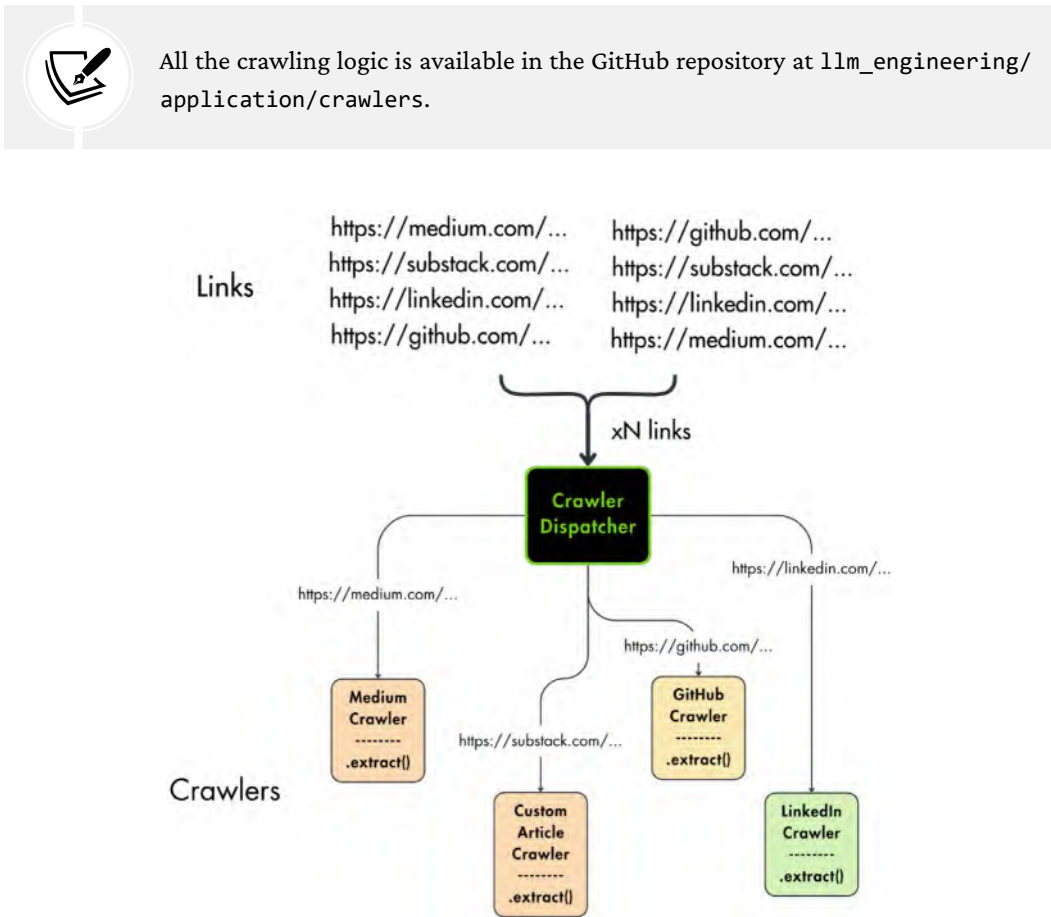
Figure 3.4: The relationship between the provided links, the CrawlerDispatcher , and the crawlers
